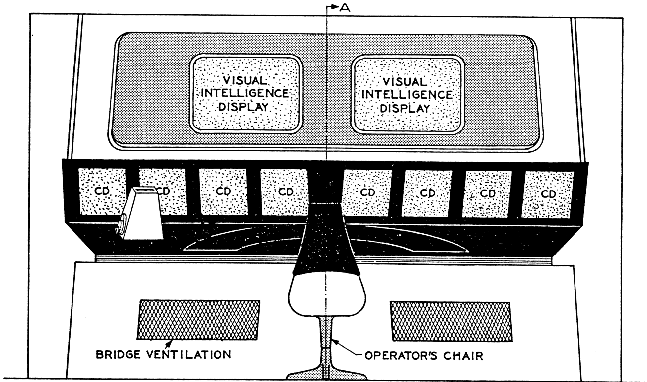
FRONT ELEVATION
